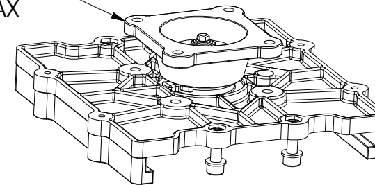
ISOMETRIC VIEW SCALE 1 / 4
