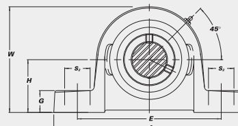
B-type Seal
