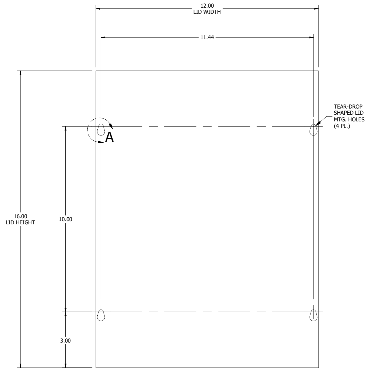
FRONT VIEW
