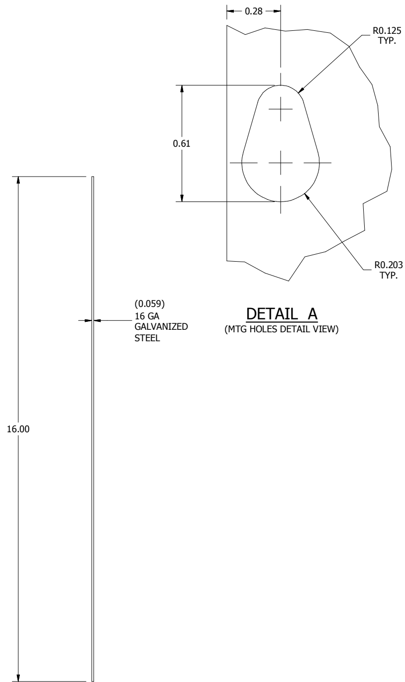
SIDE VIEW
