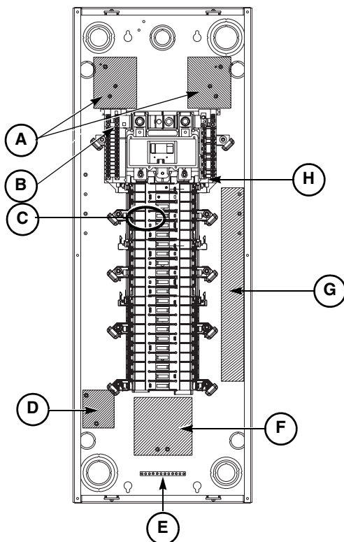
Figure 3: Indoor Intelligent Load Center Keep Out Areas
