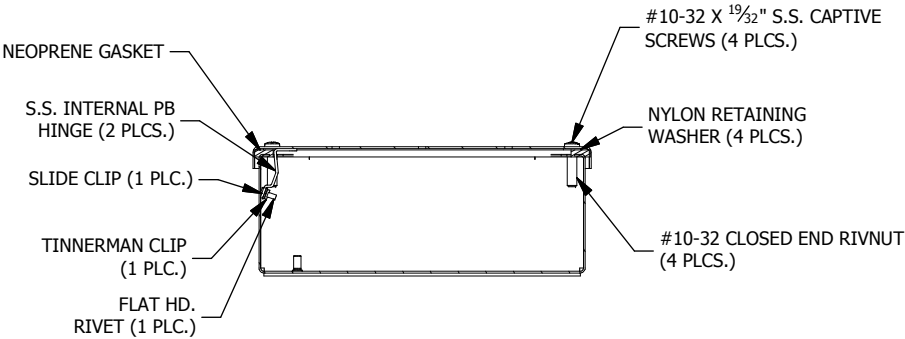
SECTION A-A (INSIDE TOP OF ENCL.)
