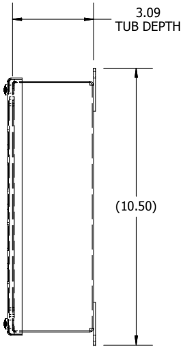
RIGHT VIEW
