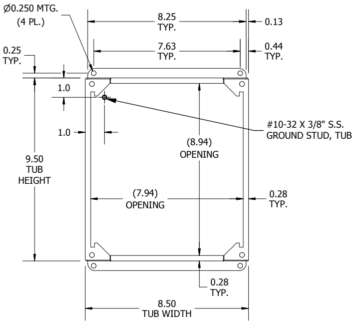
FRONT VIEW TUB
