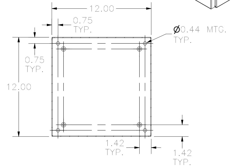
SECTION B-B (INSIDE BACK OF ENCLOSURE)
