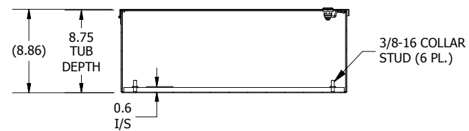
SECTION A-A (INSIDE TOP OF ENCL.)
