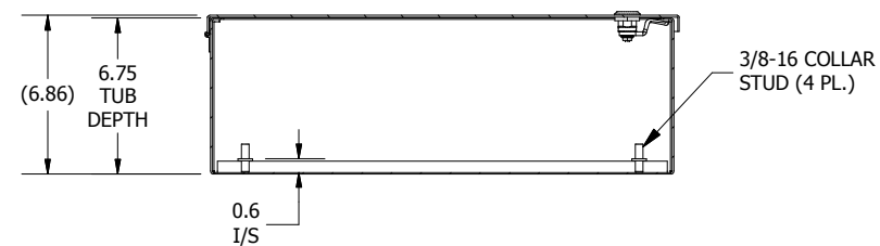
SECTION A-A (INSIDE TOP OF ENCL.)
