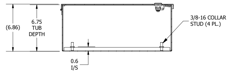
SECTION A-A (INSIDE TOP OF ENCL.)
