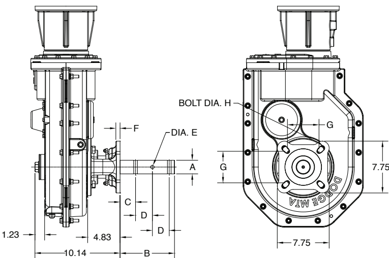
TA2115H Screw Conveyor Drive Dimensions
