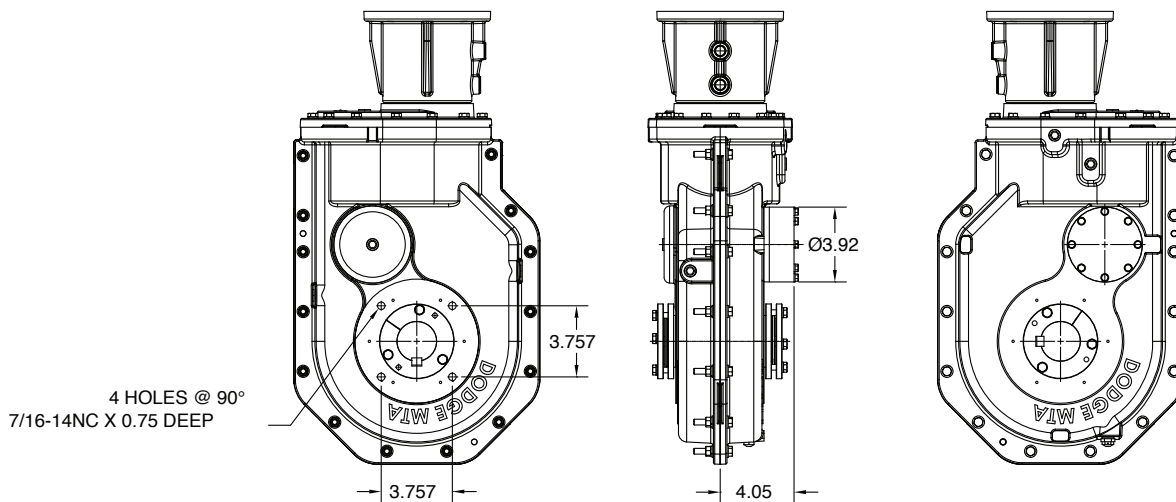
Reducer with Backstop
