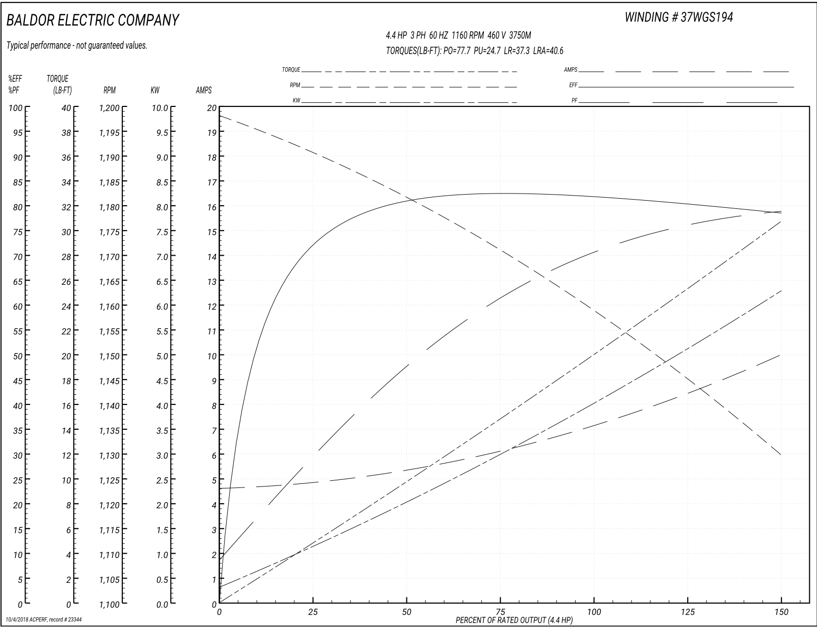
Performance Graph at 460V, 60Hz, 4.4HP Typical performance - Not guaranteed values
