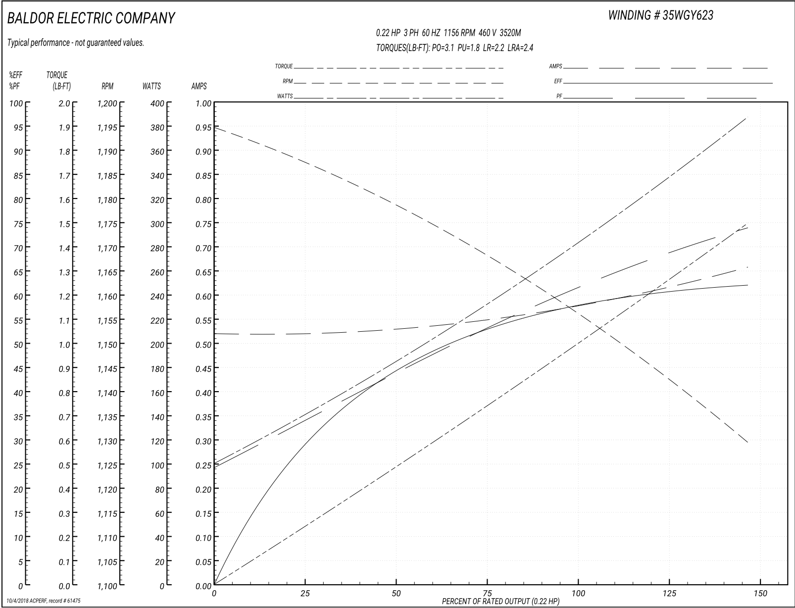
Performance Graph at 460V, 60Hz, 0.22HP Typical performance - Not guaranteed values
