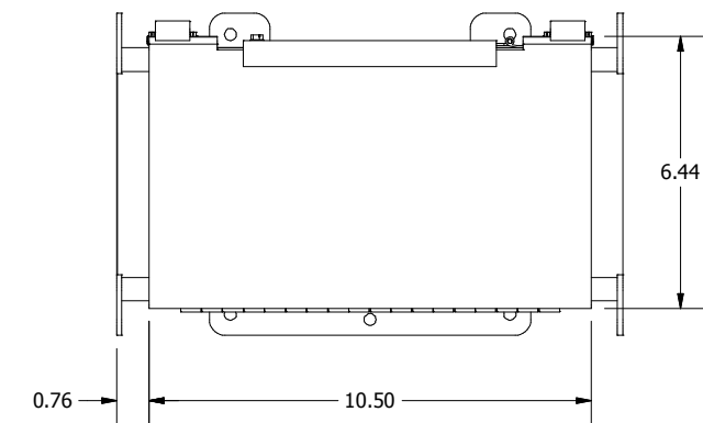
VIEW AC-AC (BACK LID VIEW)
