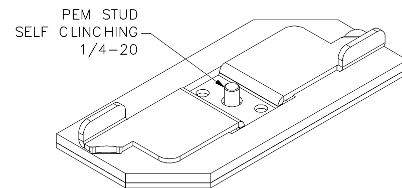
NUT REMOVED
