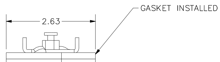
FRONT VIEW
