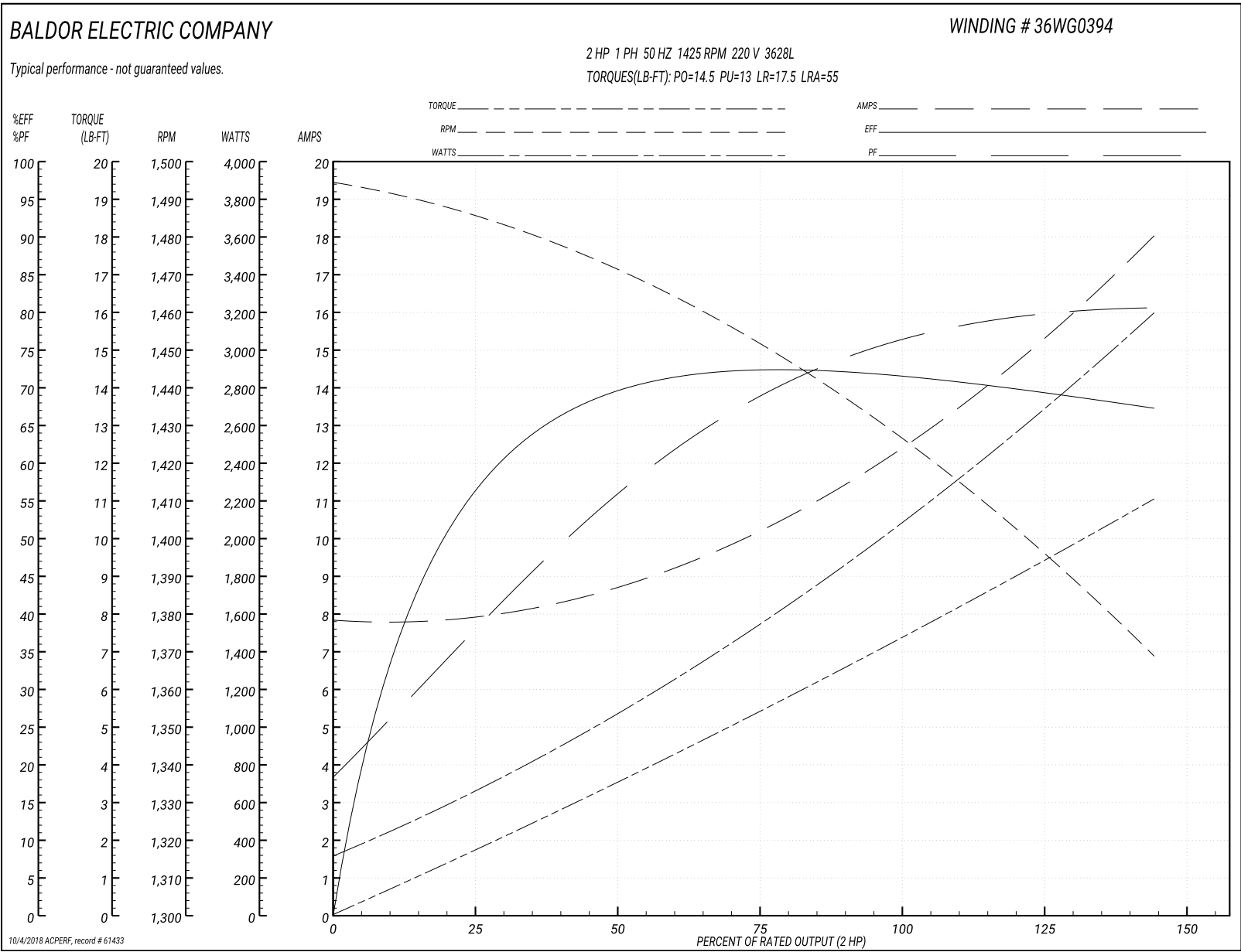
Performance Graph at 220V, 50Hz, 2.0HP Typical performance - Not guaranteed values
