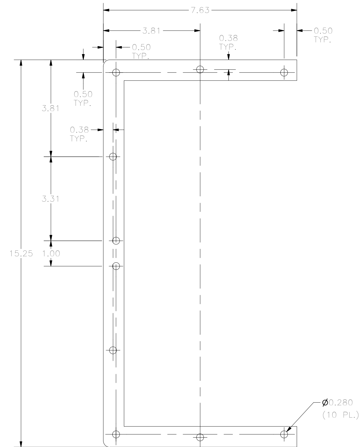
FRONT VIEW
