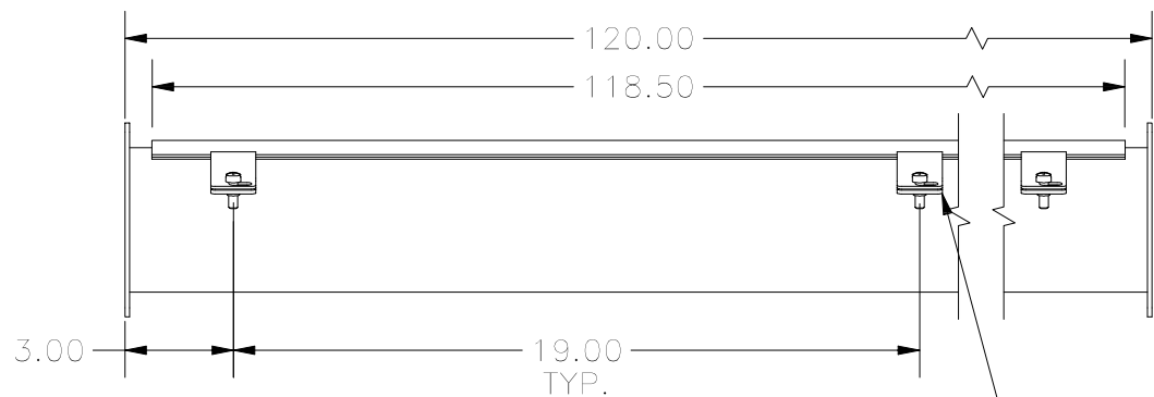
FRONT VIEW
