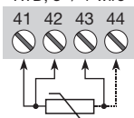
RTD, 3- / 4-wire
