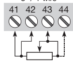
Resistance, 3- / 4-wire
