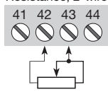
Resistance, 2-wire
