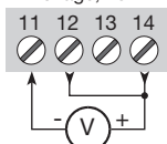
Voltage, 10 V
