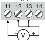
Voltage, 1 V
