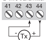
2-wire transmitter
