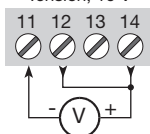
Tension, 10 V
