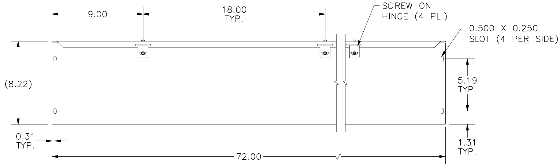
FRONT VIEW
