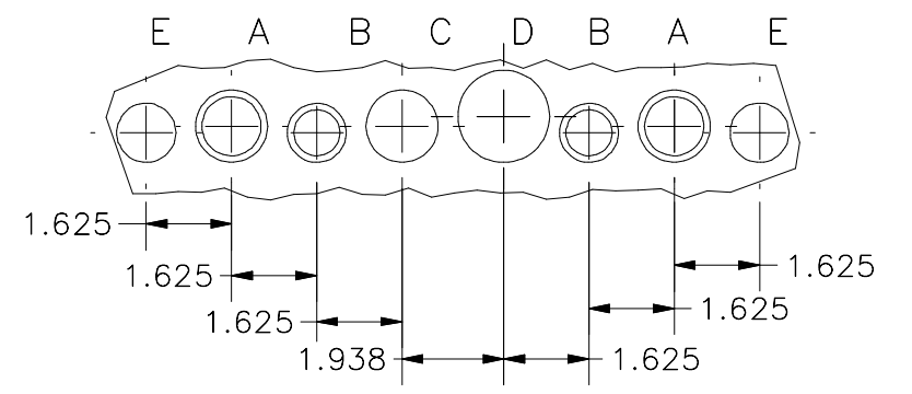
DETAIL A (4 PL. PER SIDE) K.O. PATTERN DESCRIPTION
