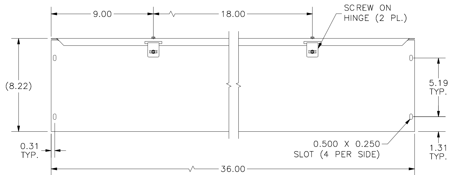
FRONT VIEW
