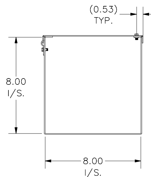
RIGHT VIEW
