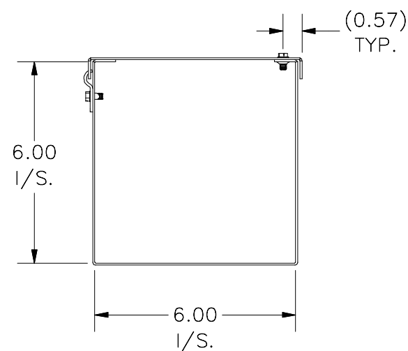
RIGHT VIEW
