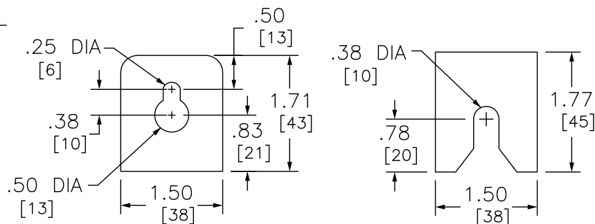
TOP MOUNTING BRACKET BOTTOM MOUNTING BRACKET
