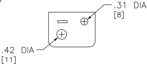
SEAL BRACKET
