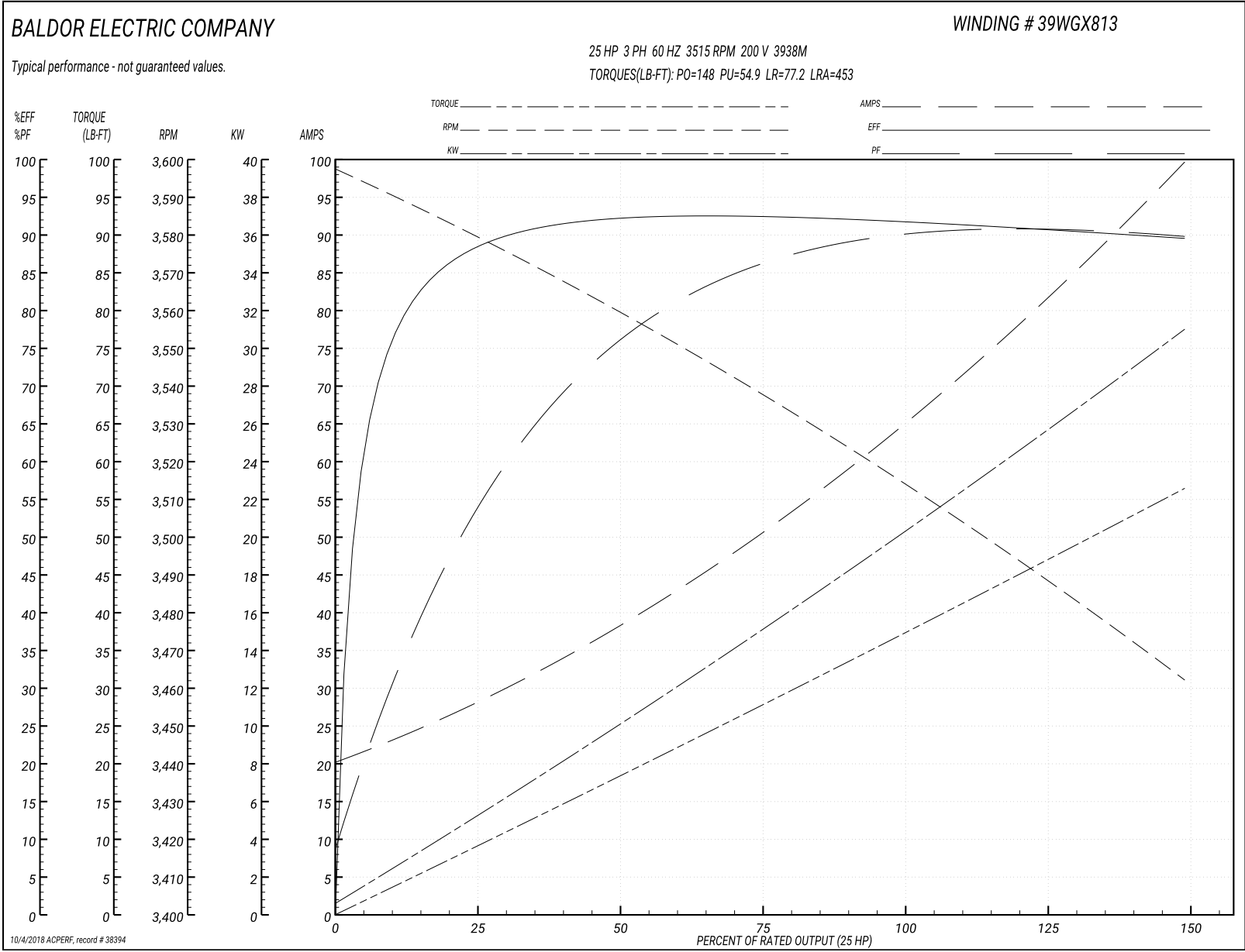
Performance Graph at 200V, 60Hz, 25.0HP Typical performance - Not guaranteed values
