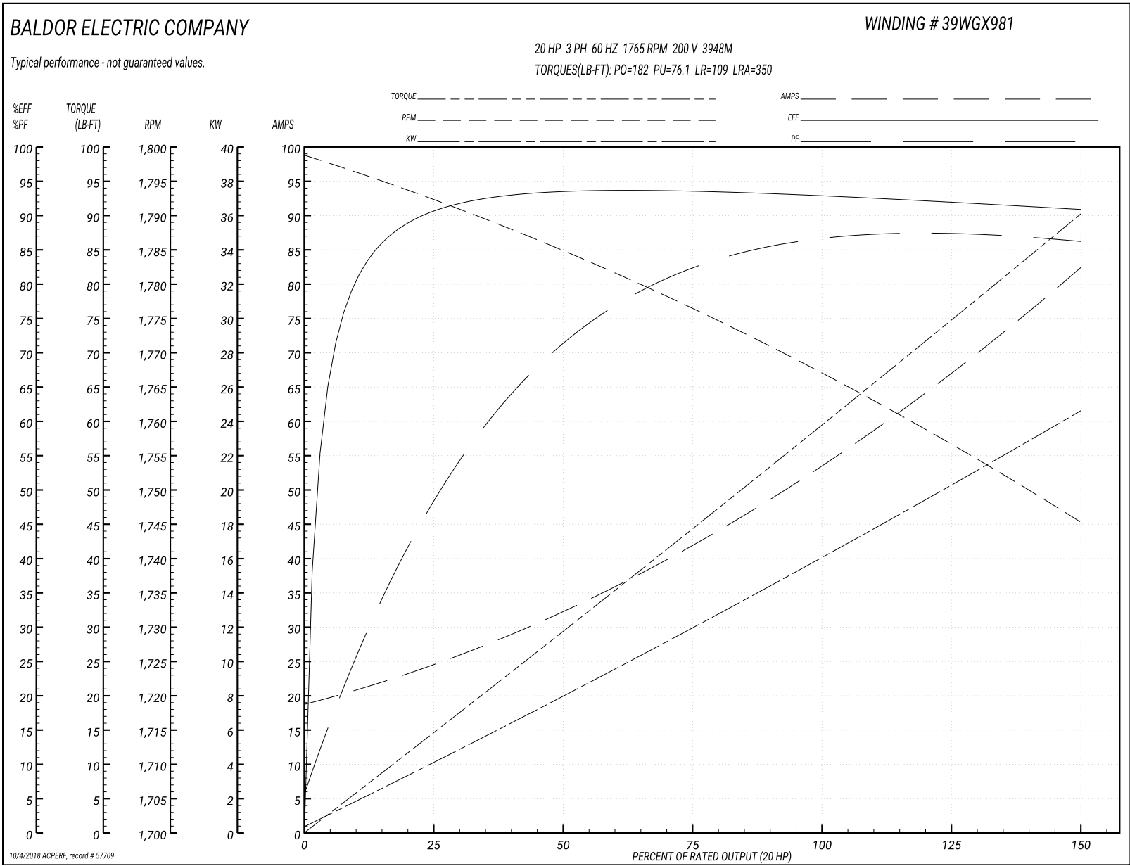
Performance Graph at 200V, 60Hz, 20.0HP Typical performance - Not guaranteed values
