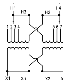
PARALLEL CONNECTION
