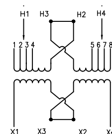
SERIES CONNECTION
