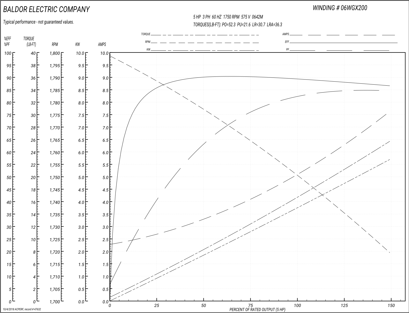
Performance Graph at 575V, 60Hz, 5.0HP Typical performance - Not guaranteed values
