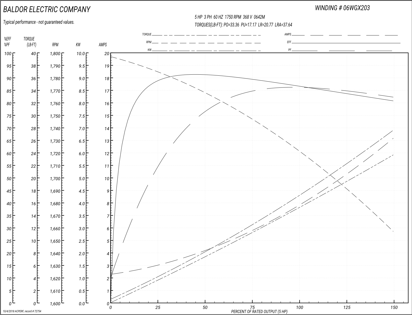
Performance Graph at 368V, 60Hz, 5.0HP Typical performance - Not guaranteed values
