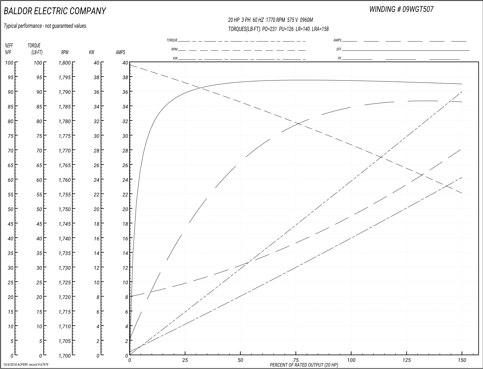
Performance Graph at 575V, 60Hz, 20.0HP Typical performance - Not guaranteed values
