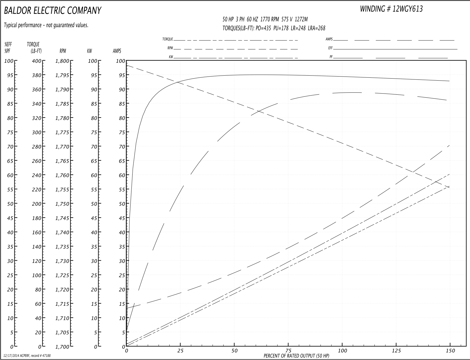
Performance Graph at 575V, 60Hz, 50.0HP Typical performance - Not guaranteed values
