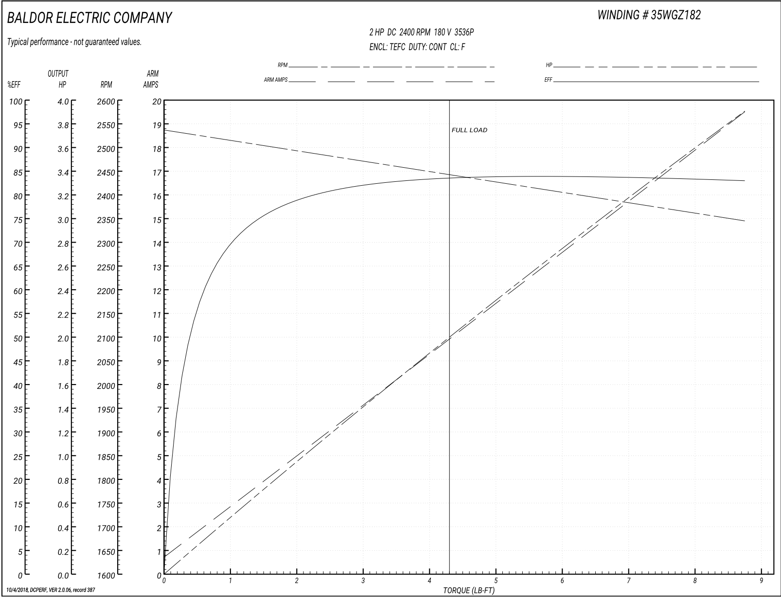
Performance Graph at 180.0 Arm V, 2.0HP Typical performance - Not guaranteed values
