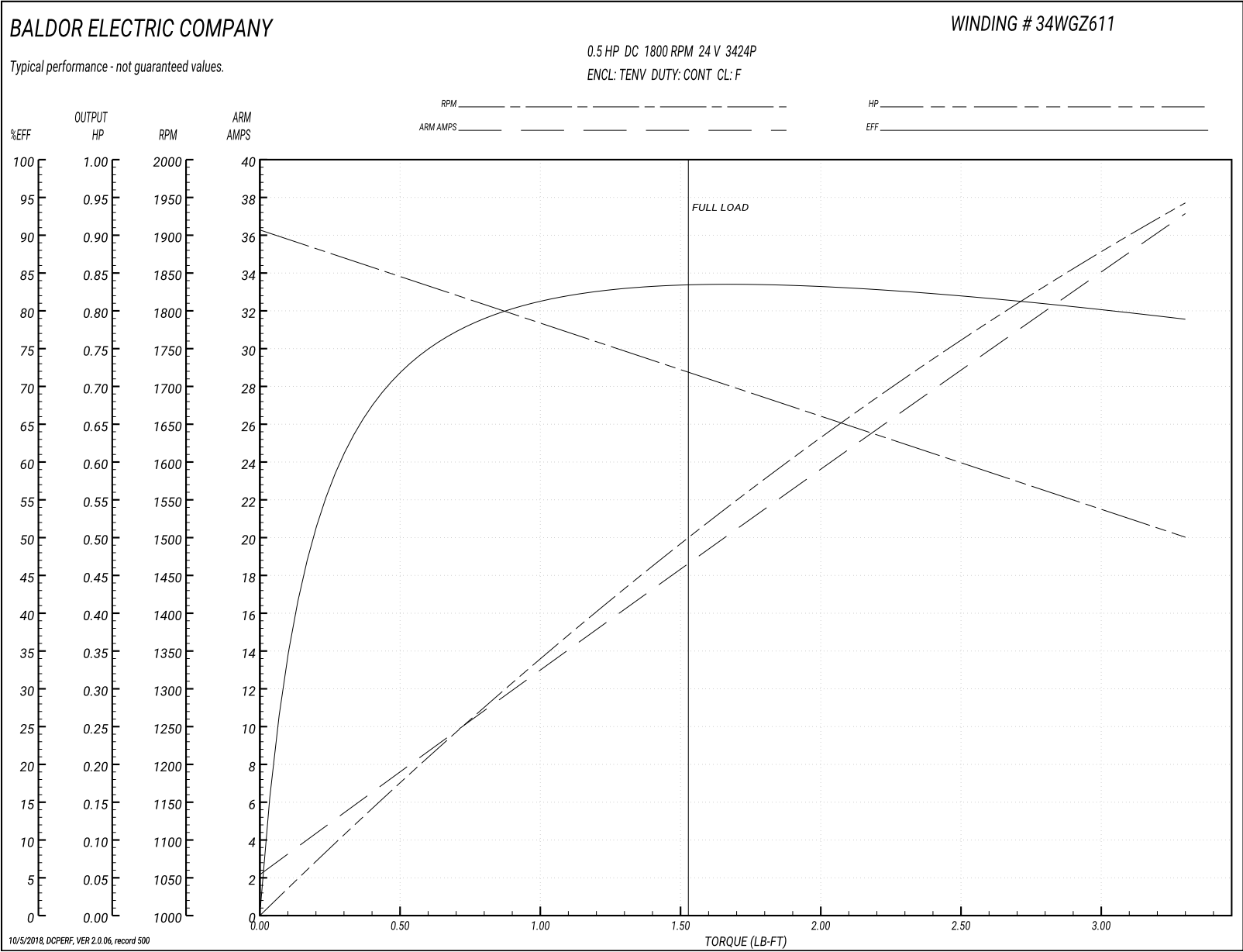
Performance Graph at 24.0 Arm V, 0.5HP Typical performance - Not guaranteed values
