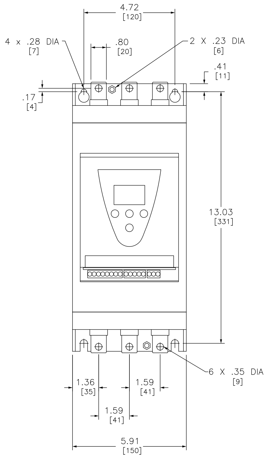
FRONT
