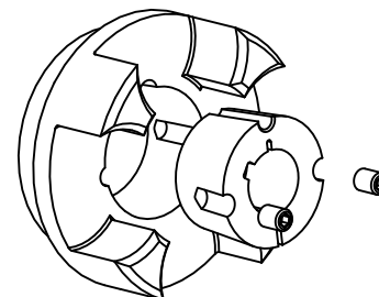
Front Mount
