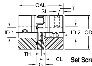
Clamping Type
