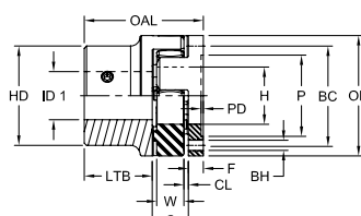
CJSFH Design
