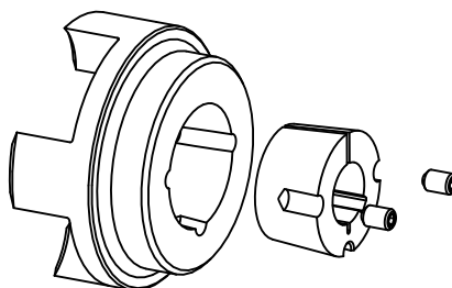
Reverse Mount
