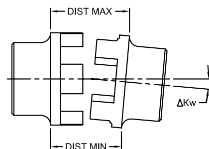
Angular Displacement
