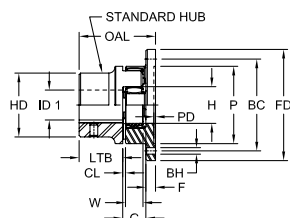
CJLFH Design
