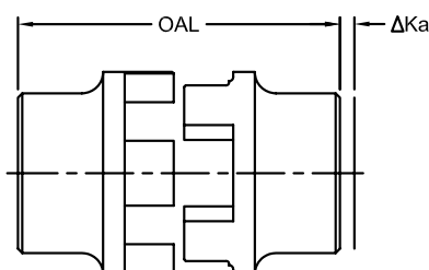
Axial Displacement
