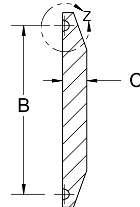
SECTION Y-Y
