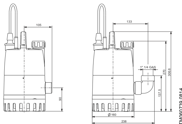
Fig. 6 Pump dimensions
