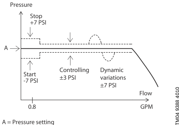
Fig. 5 System function
