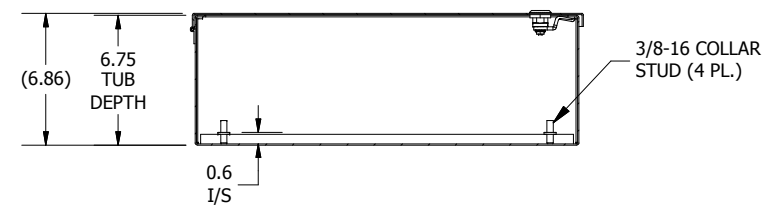
SECTION A-A (INSIDE TOP OF ENCL.)
