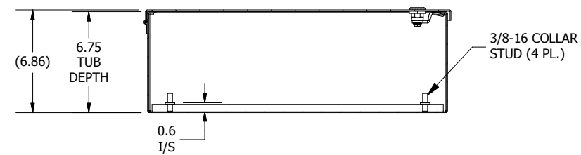
SECTION A-A (INSIDE TOP OF ENCL.)
