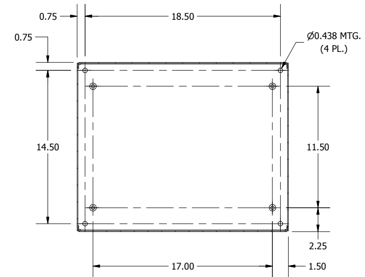
SECTION B-B (INSIDE BACK OF ENCL.)
