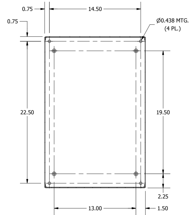
SECTION B-B (INSIDE BACK OF ENCL.)
