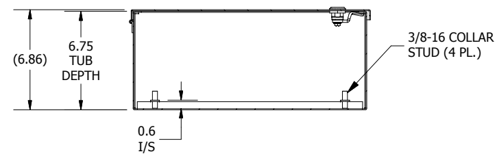
SECTION A-A (INSIDE TOP OF ENCL.)
