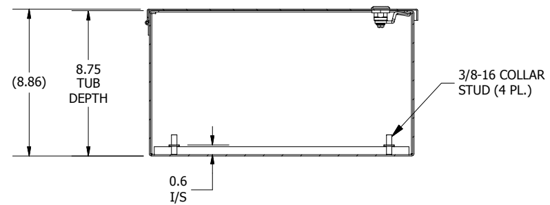
SECTION A-A (INSIDE TOP OF ENCL.)
