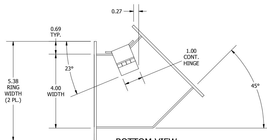
BOTTOM VIEW
