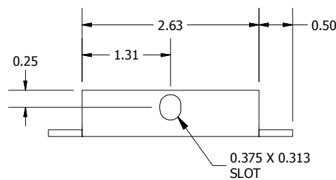
TOP PIECE FRONT VIEW
